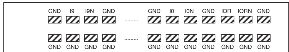
Figure 2-1. Input Data Connector
